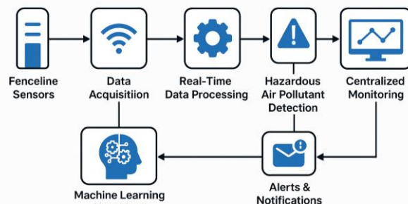
Figure 1. Fenceline sensor detection and notification framework
