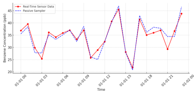
Figure 2. Real-Time vs Passive Sampler Benzene Concentration
